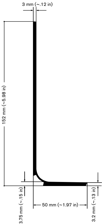
S 3019 D For floor covering thickness from 3 to 3.5 mm (~.12 in to .14 in)
