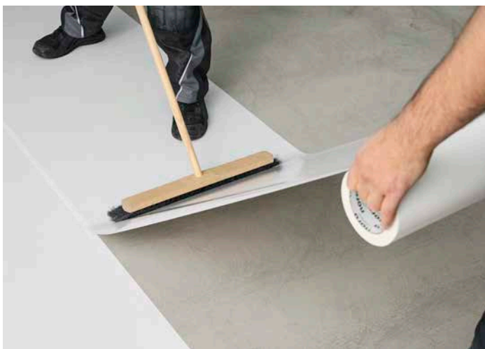
1) Roll out nora dryfix mr onto the substrate
