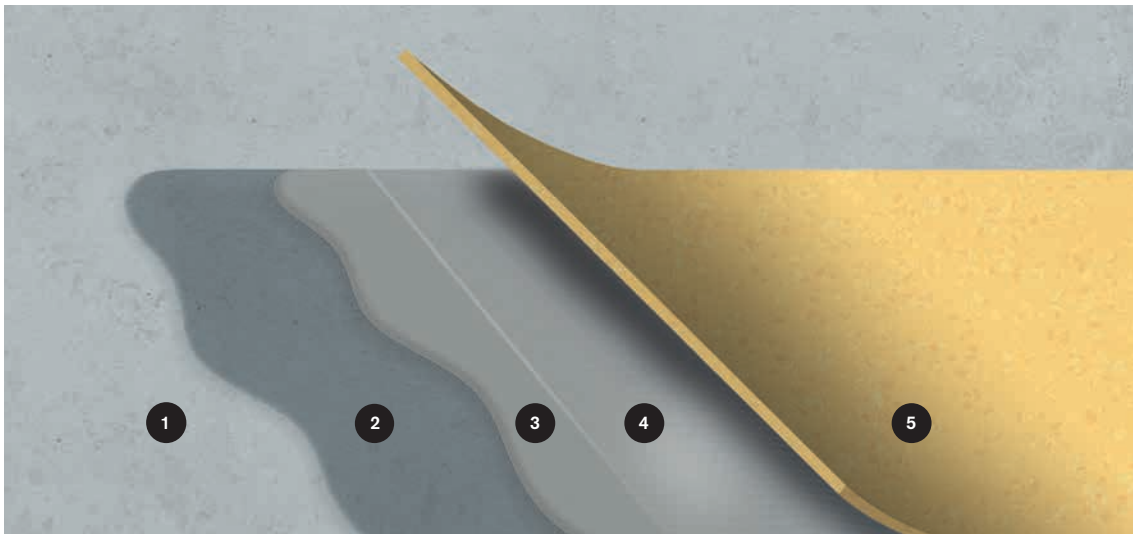
1 Substrate 2 Primer (where needed) 3 Leveler (where needed) 4 nora dryfix mr 5 nora floor covering
